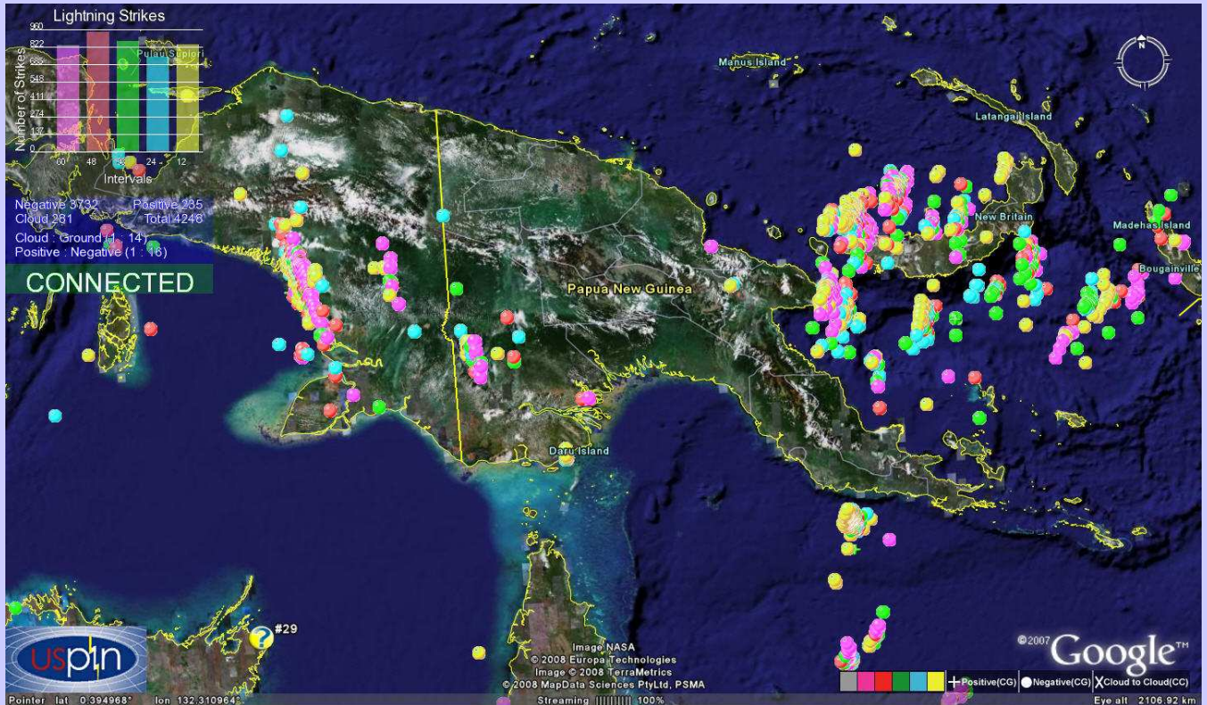
Data from the Global Lightning Network in Google Earth top image – storm cell representation of lightning bottom image – display of individual lightning events
